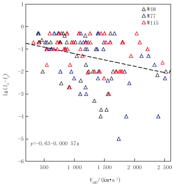
图 7 SEP 通量背景值与峰值的比与对应 CME 速度的相关性 Fig.7 Correlation between ratio of background value to peak value of SEP flux and corresponding CME velocity
