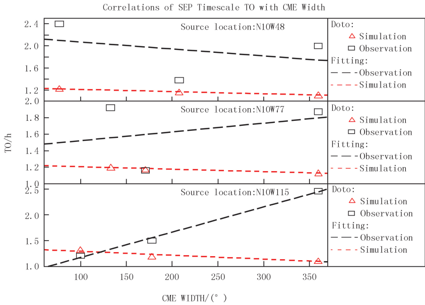
图 5 数值模拟方法下 SEP 时间尺度 TO 与 CME 宽度关系数值模拟与观测对比图 Fig.5 Comparison of SEP timescale TO and CME widths with simulation and observation under numerical simulation method
