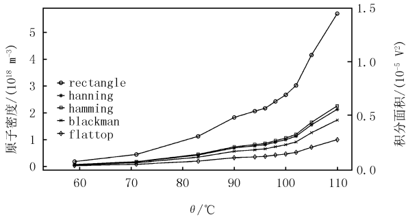
图6 原子密度/共振峰积分面积在不同窗函数下随温度的变化 Fig.6 The integral area of resonance peak(the atomic density) versus temperature under different window functions
