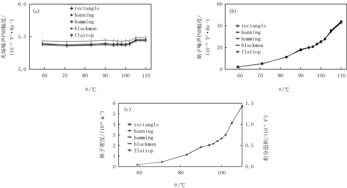
图7 窗口效应修正后,光场噪声(a)、原子自旋噪声(b)及原子密度(c)在不同窗口函数作用下,随温度的变化 Fig.7 Optical noise(a), spin noise(b) and atomic density(c) versus temperature under different window functions, and corrected by correction factors
