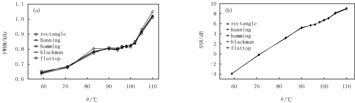
图5 半高全宽(a)和信噪比(b)在不同窗函数下随温度变化图 Fig.5 The full width half maximum(a) and the signal-to-noise ratio(b) versus temperature under different window functions
