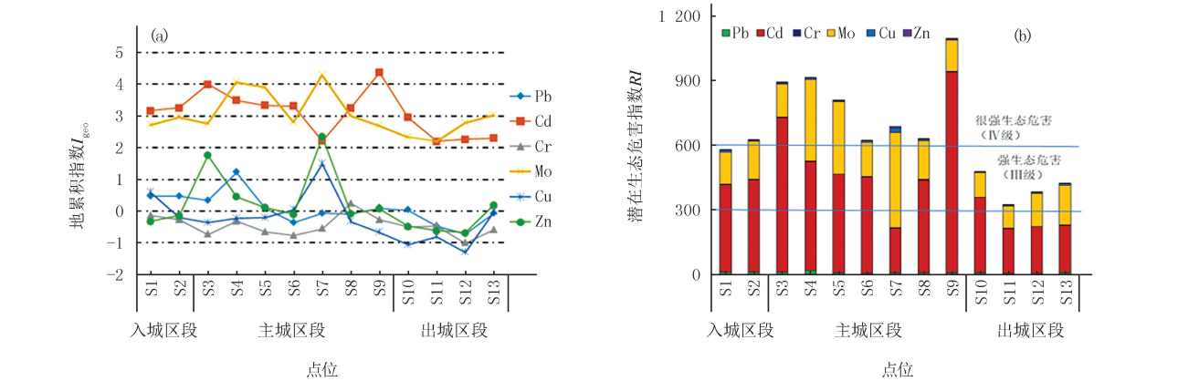
图3 地累积指数(a)和潜在生态风险评价指数(b) Fig.3 Geo-accumulation index(a) and potential ecological risk index(b) of heavy metals in sediments
