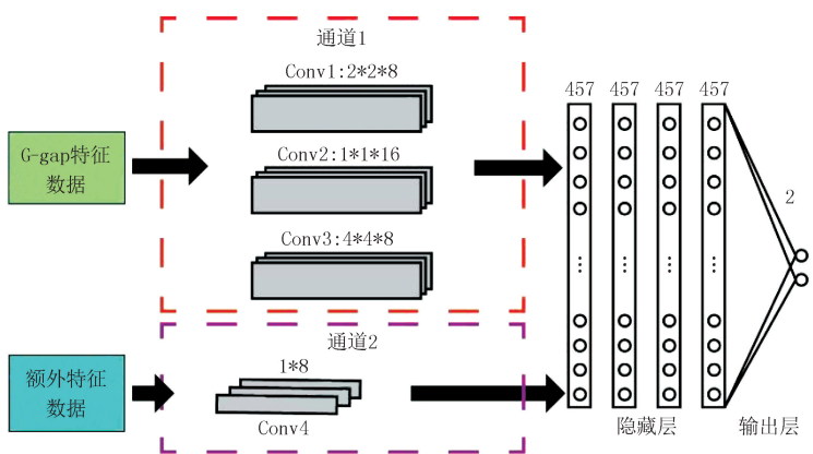
图5 SCNN模型整体结构图 Fig.5 The overall structure of the SCNN model
