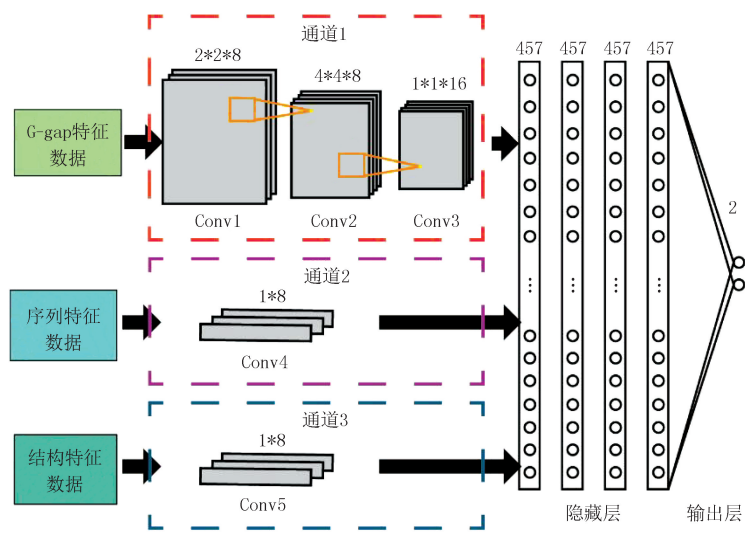
图4 DTcCNN模型整体结构图 Fig.4 The overall structure of the DTcCNN model
