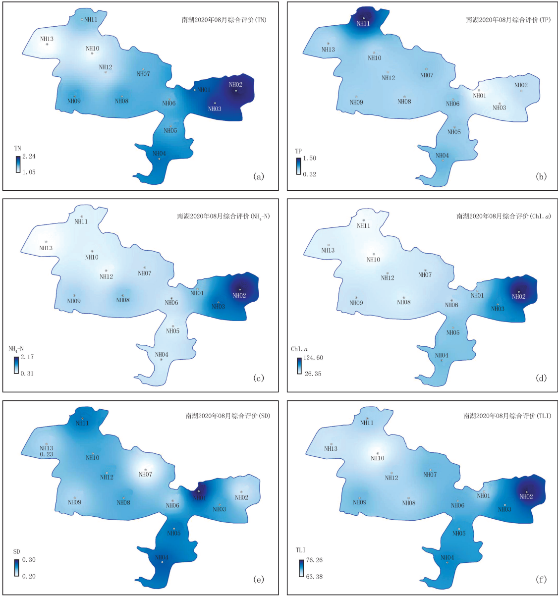
图3 南湖水质的时空变化 Fig.3 Temporal and spatial changes of water quality in South Lake
