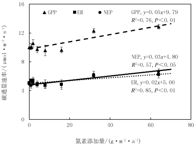
图2 温带典型草原生态系统碳通量与氮素添加速率之间关系 Fig.2 Relationships between ecosystem carbon fluxes and nitrogen addition rates in a typical temperate steppe
